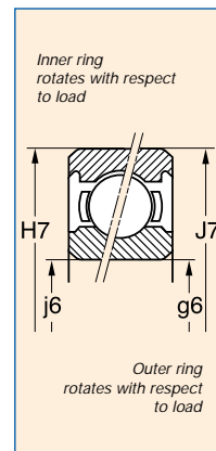
Recommended Fitting Tolerance
